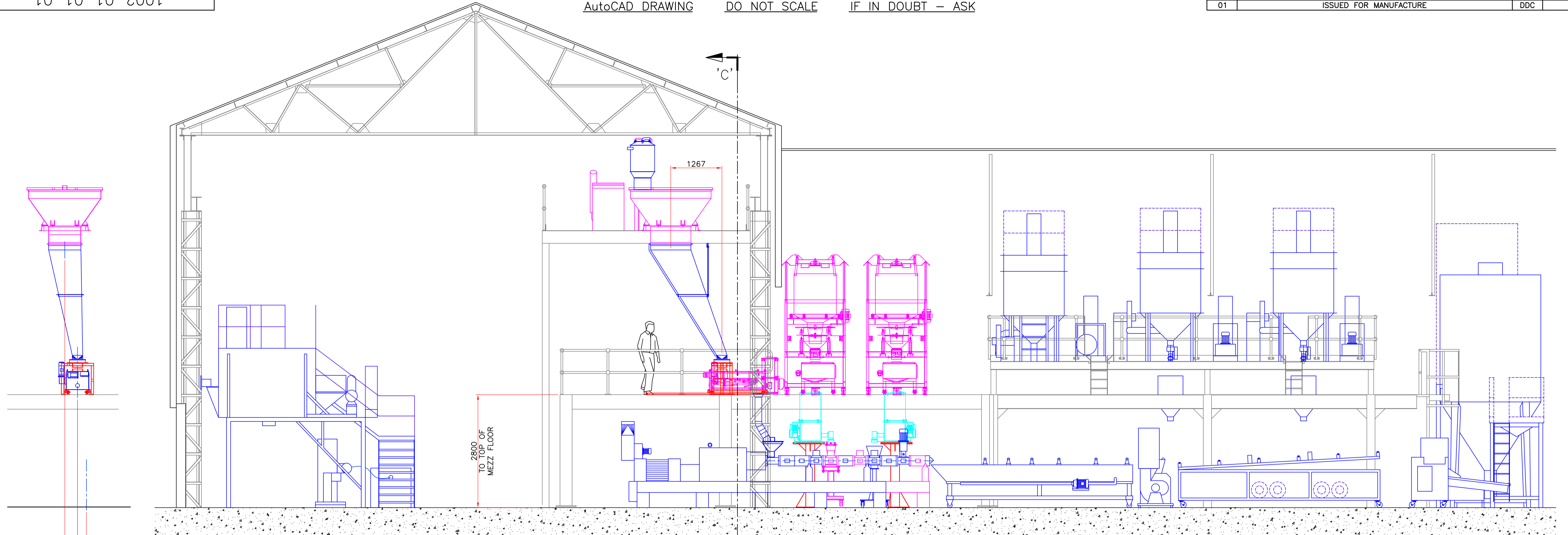
SECTION 'A-A' SECTION THRO' TSK-90 4234
